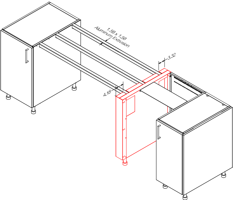
OBX OCS R installed in middle of run with cabinet.
