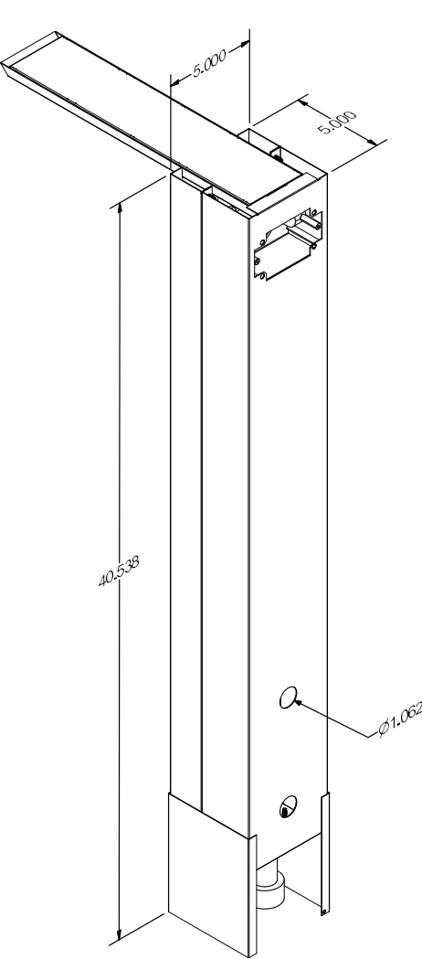
OCPS41E (electrical cutout)
