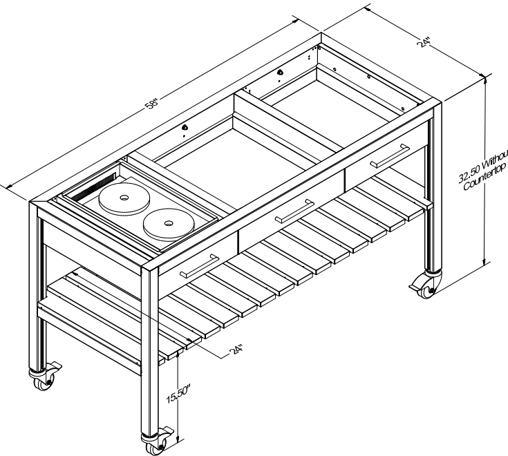
Cosmopolitan Table Cook With Casters ADA
