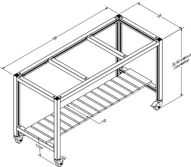
Cosmopolitan Table Dining ADA With Casters
