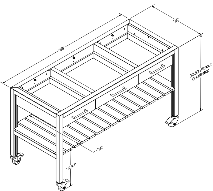
Cosmopolitan Table Storage ADA With Casters
