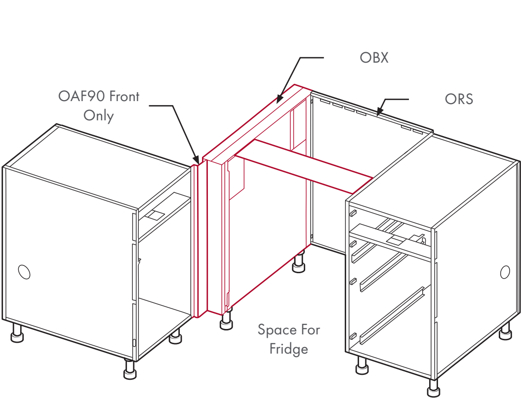
Example of how to place refrigerator next to corner.
