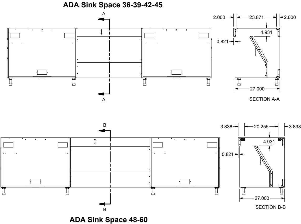
OBSxx00 ADA SINK SPACE configuration variations
