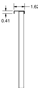
Pull tab placement on slab drawer.
