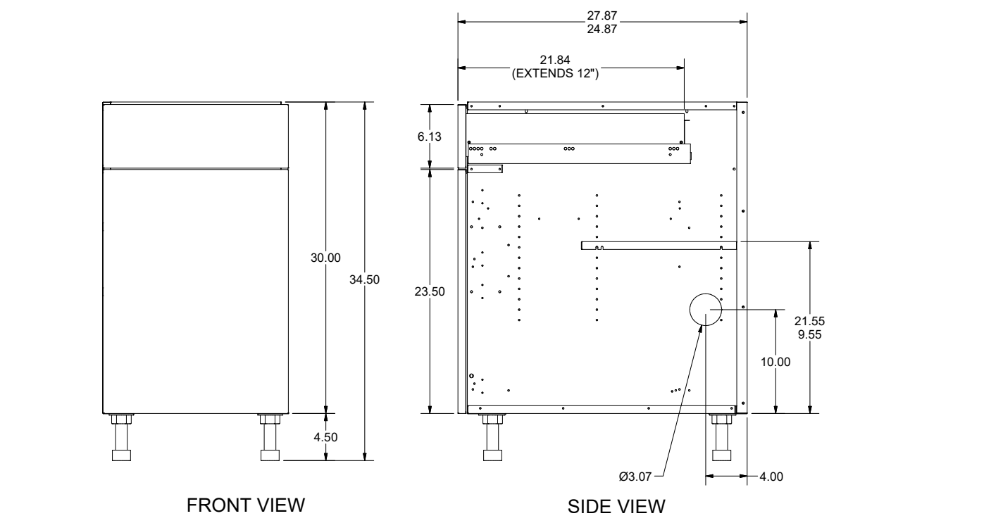
Typical cabinet foot location.
