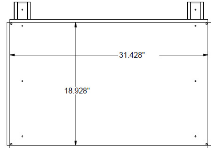
Ex. OSH36PCHEST, installs in 36"W cabinet
