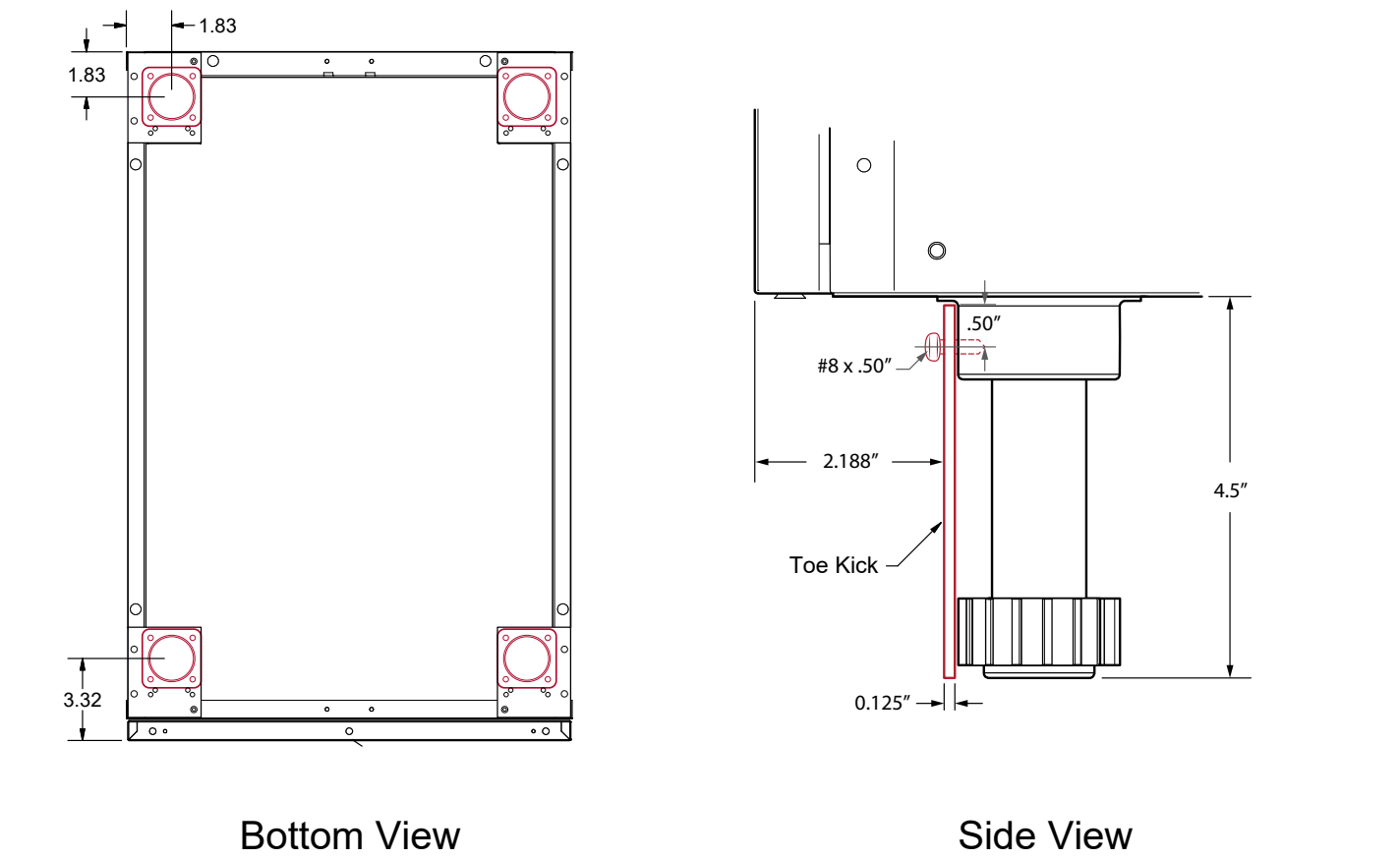
Typical cabinet foot location.
