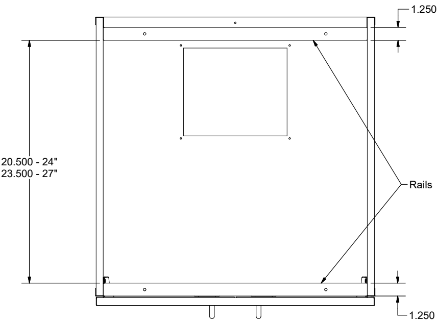
Plan View
