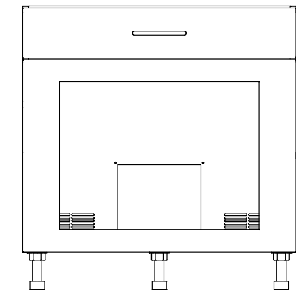
front view with trim
