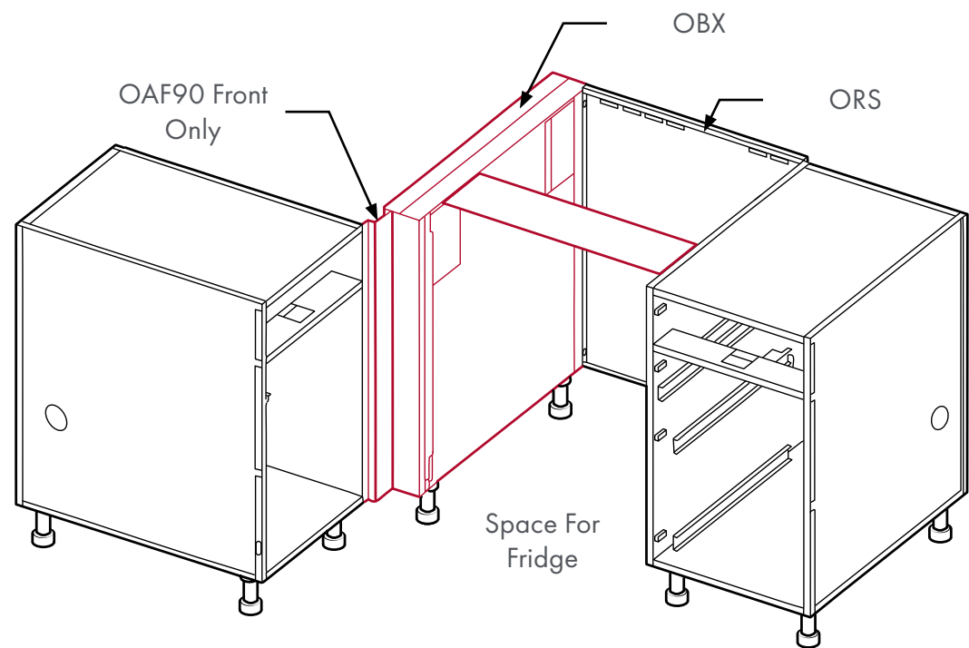
Example of how to place refrigerator next to corner.
