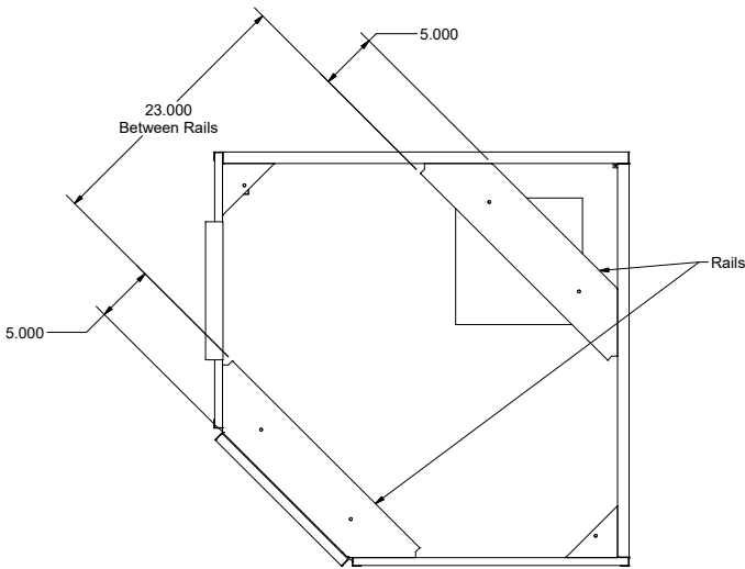
DCBS36 Cabinet Sink Spacing
