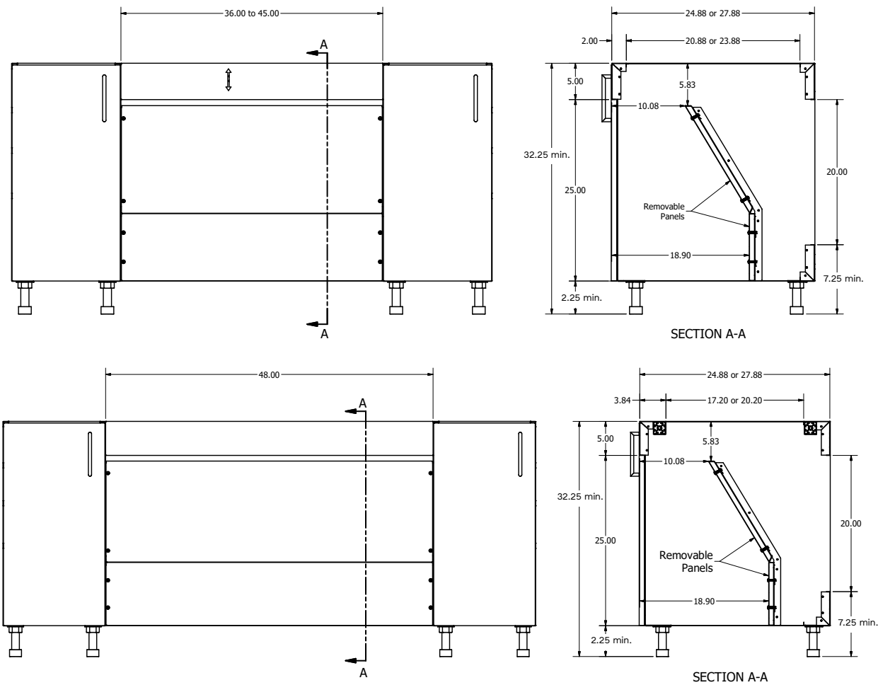
OBSxx00 ADA SINK SPACE configuration variations
