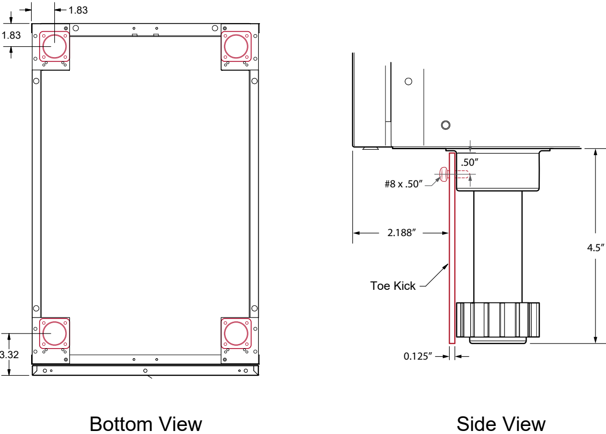
Typical cabinet foot location.
