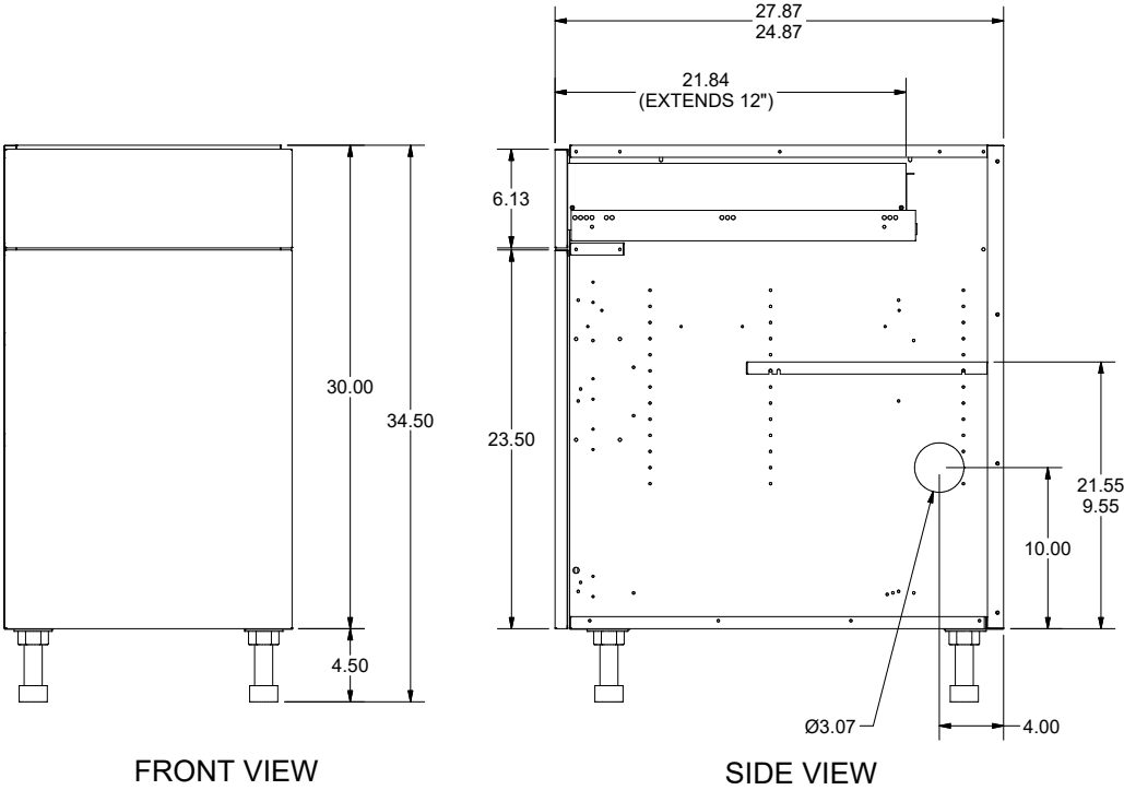
Typical cabinet foot location.
