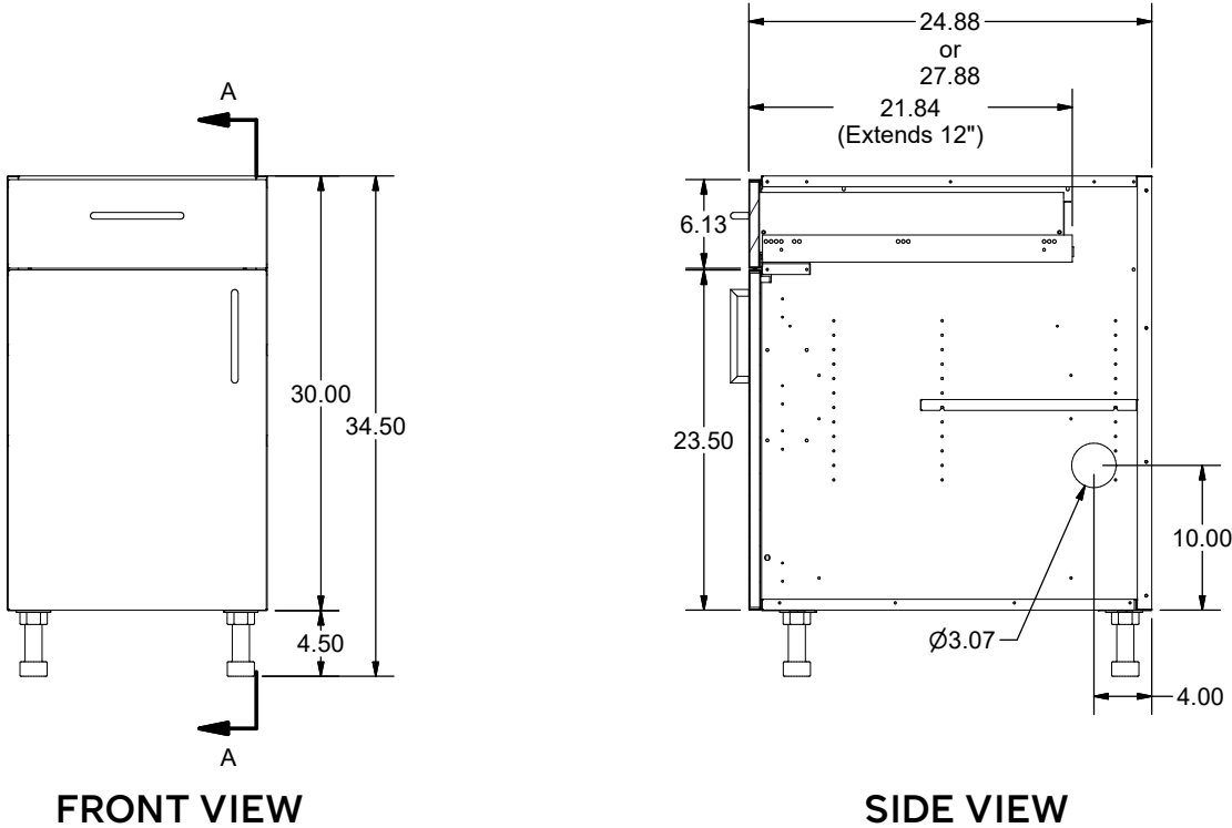
Typical cabinet foot location.
