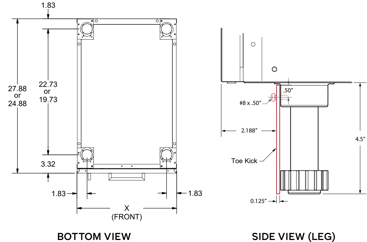
Typical cabinet foot location.
