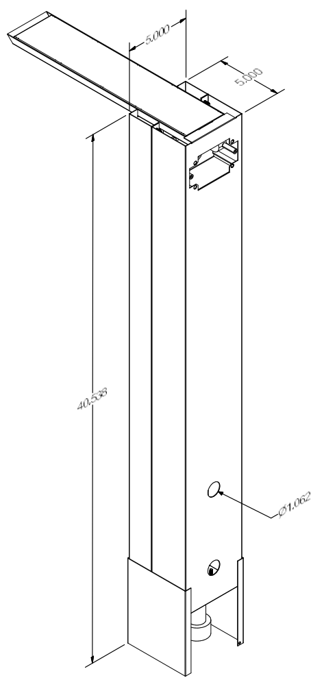
OCPS41E (electrical cutout)
